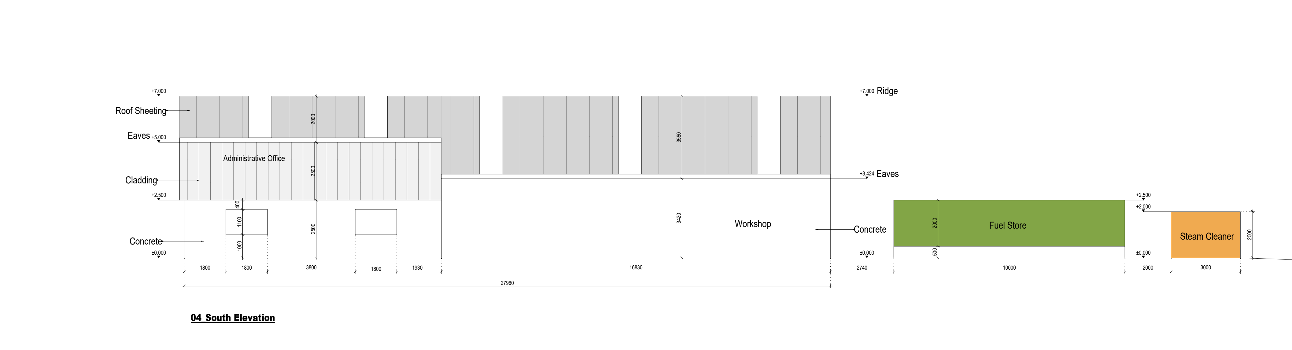
Main Office Elevations Scale 1:100
